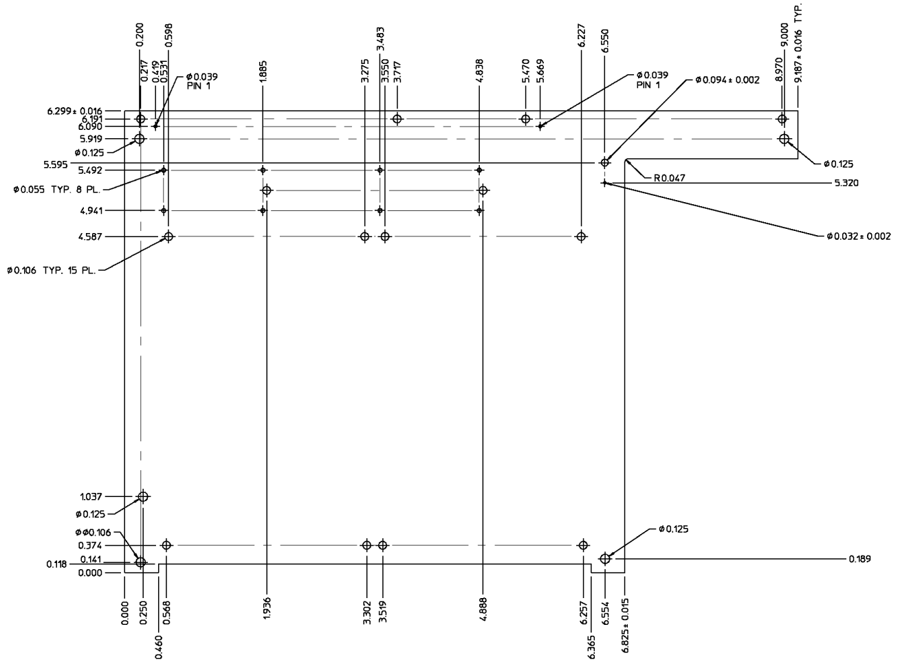
Figure 4-18 PMC Expansion Adapter
