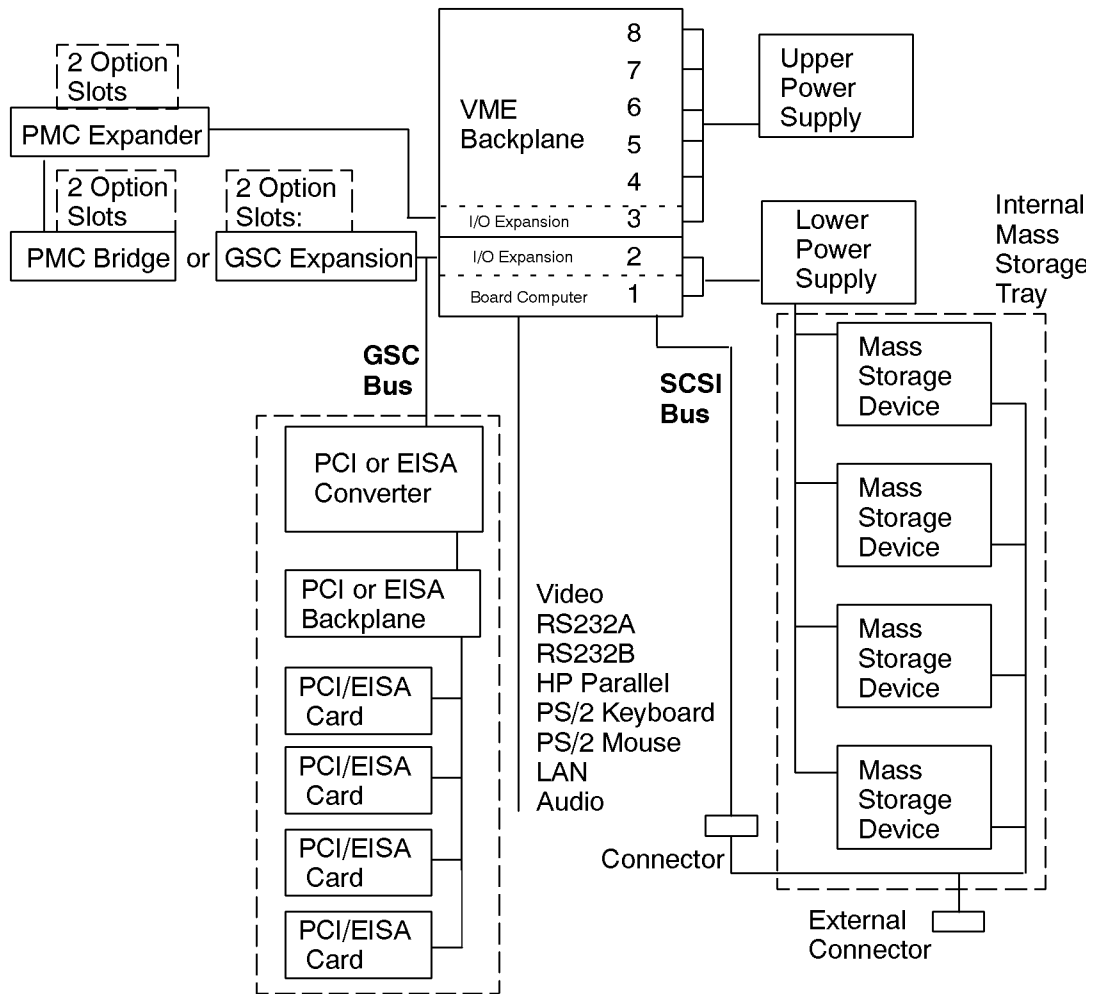
Figure 1-8 Model 748 Functional Block Diagram
