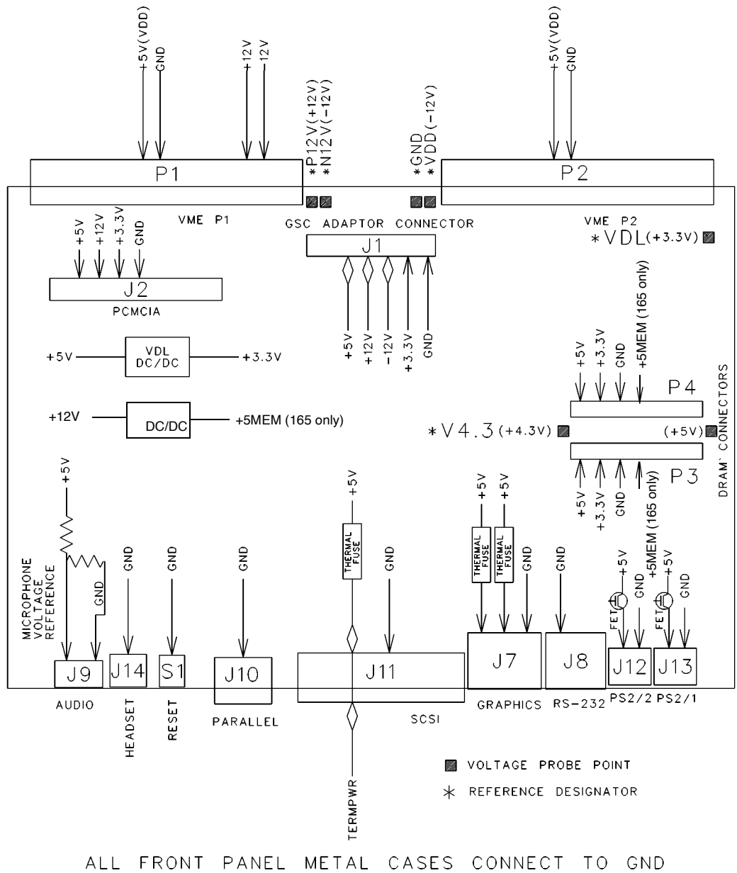
Figure 6-2 Model 744 Board Computer Power Distribution Diagram
