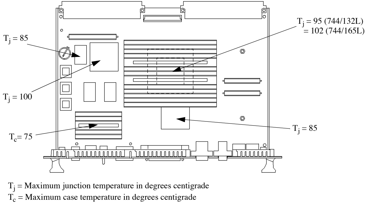
Figure 4-4 Model 744 Integrated Circuit Case Temperature Limits
