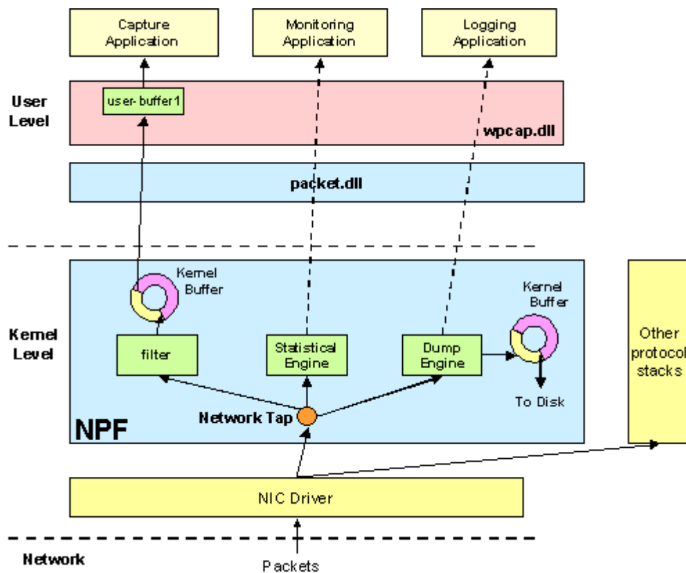
Figure 30: NPF Device Driver
