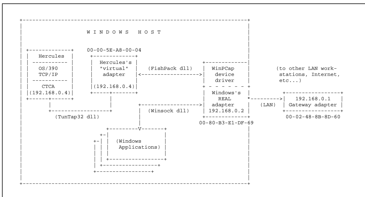
Figure 32: CTCI-W32 Implementation
