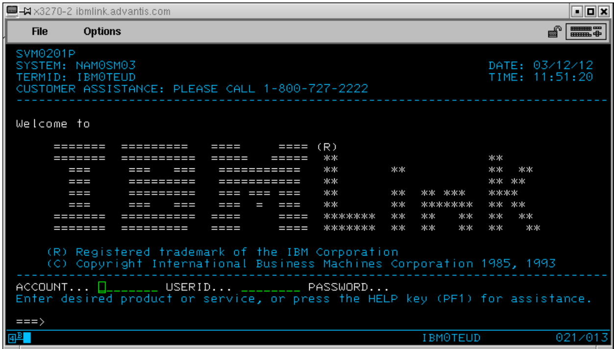
Figure 36: x3270 Window
