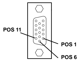
Controller Connector (female)
