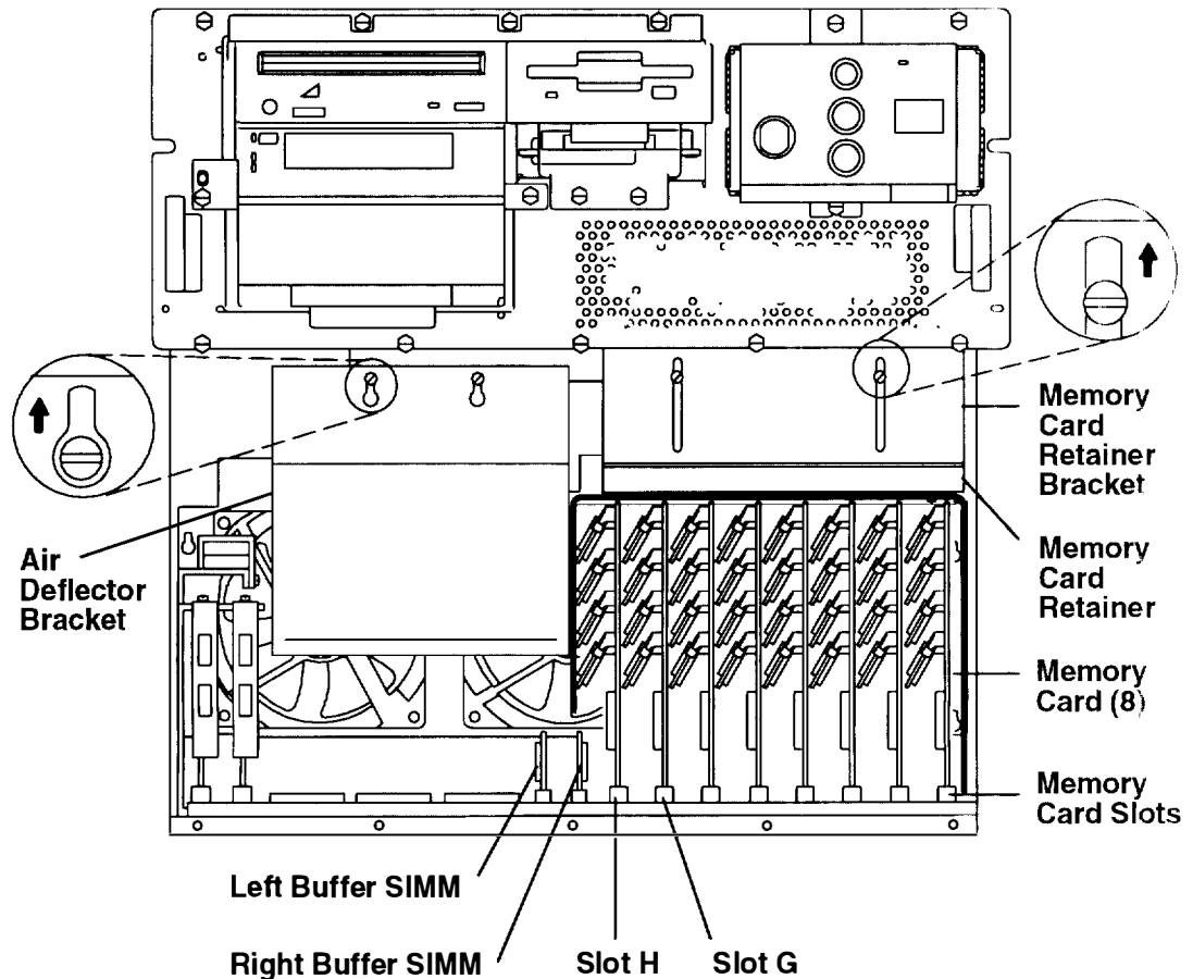
Front of CPU-Media Enclosure
