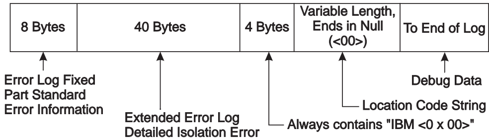
Figure 1. Standard IBM CHRP error log format
