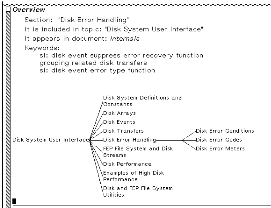
Figure 93. Document Examiner display of Show Overview of topic "Disk Error Handling".
