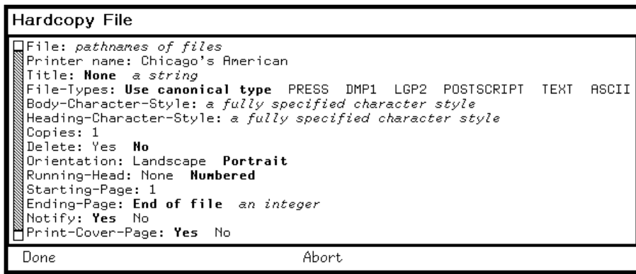
Figure 84. The Hardcopy Menu
