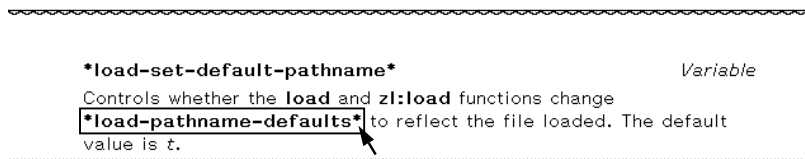
Figure 92. The names of Lisp objects displayed in the viewer are mouse-sensitive.
