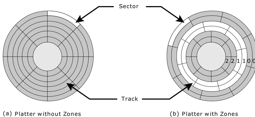
Figure 2-6: Zoned bit recording
