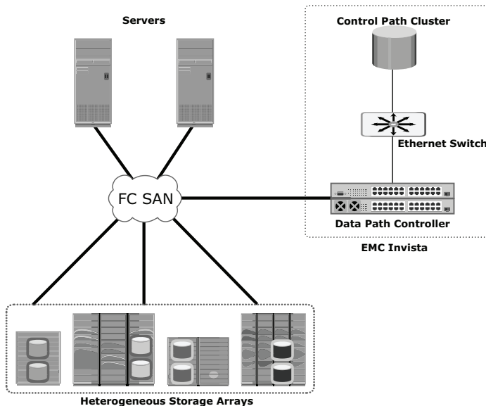
Figure 10-9: Invista's hardware components
