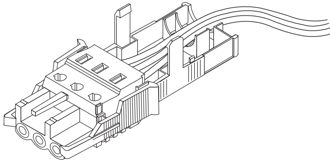
Figure 5-10 Routing the Wires Out of the Bottom Portion of the Strain Relief Housing
