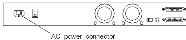
Figure 4-10 Netra st D130 Rear View (AC Version)
