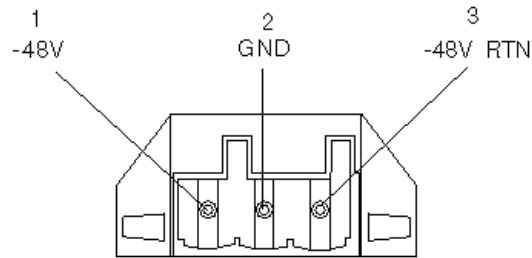
Figure 5-4 Power Connector on the DC Power Supply
