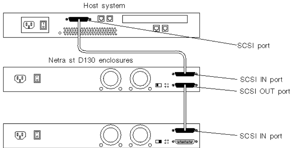
Figure 6-3 Daisy-Chaining Netra st D130 Storage Enclosures
