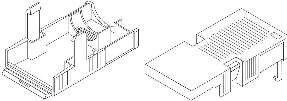
Figure 5-2 Strain Relief Housing
