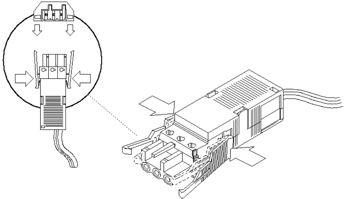
Figure 6-8 Disconnecting the DC Input Power Cable from the DC Connector
