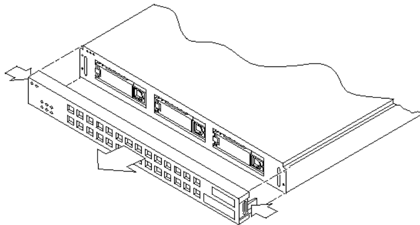
Figure 4-2 Removing the Front Panel
