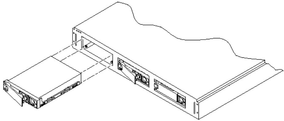
Figure 7-2 Adding a Disk Drive
