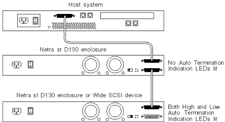
Figure 4-8 Auto Termination Indication LEDs Lit in UltraSCSI or Wide SCSI Daisy-Chain
