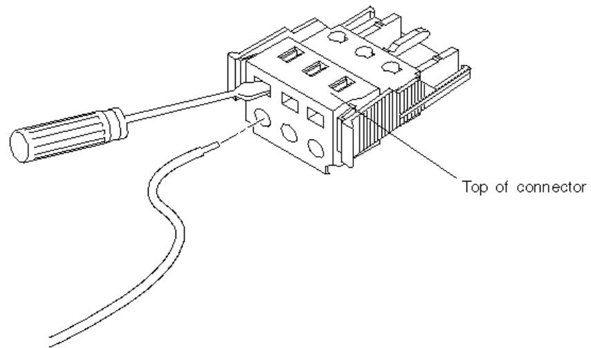
Figure 5-7 Opening the DC Connector Cage Clamp Using a Screwdriver
