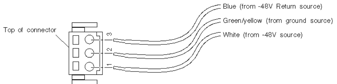
Figure 5-8 Assembling the DC Input Power Cable
