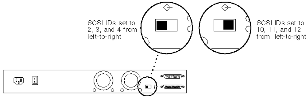
Figure 6-1 Locating the SCSI ID Switch
