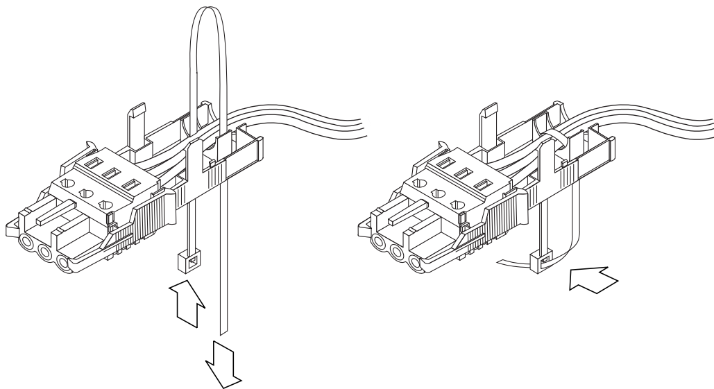
Figure 5-11 Securing the Wires to the Strain Relief Housing
