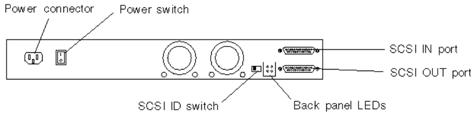
Figure 4-4 Netra st D130, Rear View
