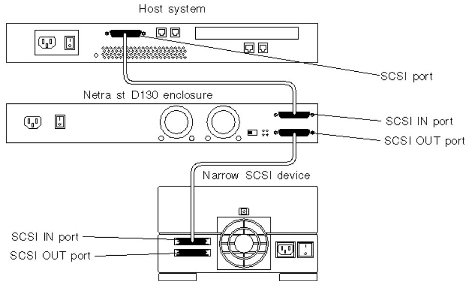
Figure 6-4 Daisy-Chaining a Netra st D130 Storage Enclosure with a Narrow SCSI Device
