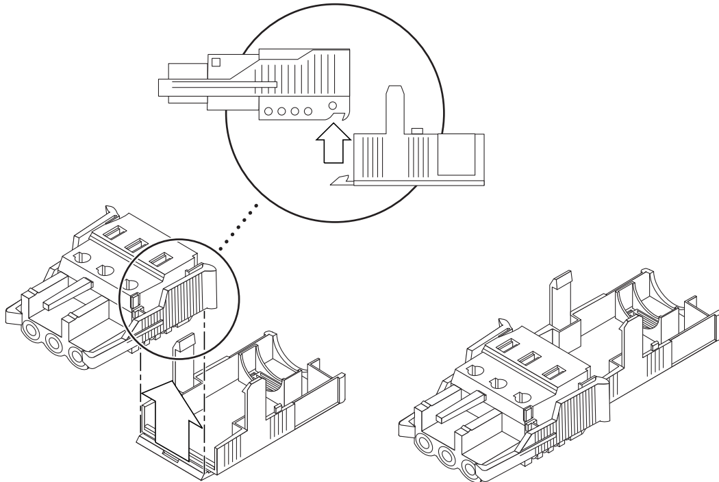
Figure 5-9 Inserting the Bottom Portion of the Strain Relief Housing
