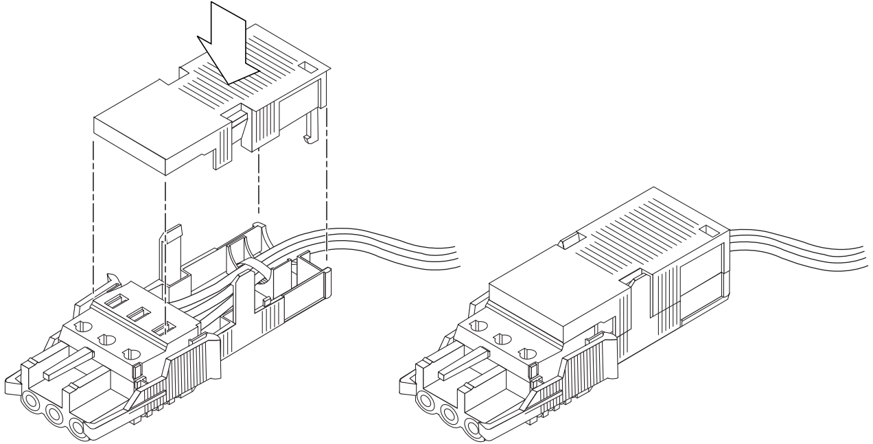
Figure 5-12 Assembling the Strain Relief Housing
