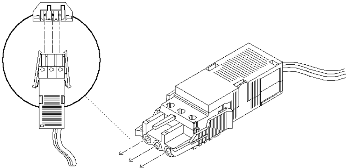
Figure 6-7 Connecting the DC Input Power Cable to the DC Connector
