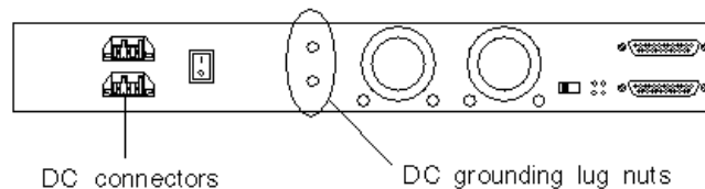
Figure 6-6 Connecting the DC Grounding Cable
