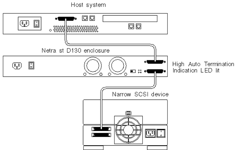
Figure 4-9 Auto Termination Indication LEDs Lit in a Narrow SCSI Daisy-Chain
