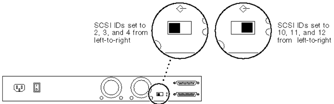
Figure 4-6 SCSI ID Switch
