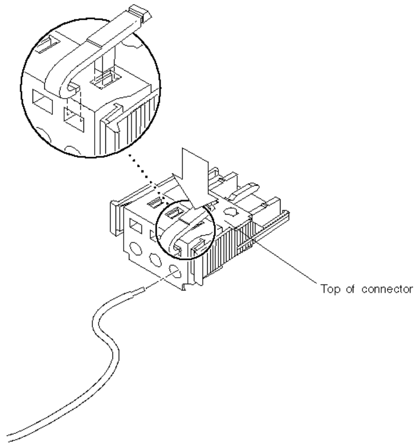
Figure 5-6 Opening the DC Connector Cage Clamp Using the Cage Clamp Operating Lever
