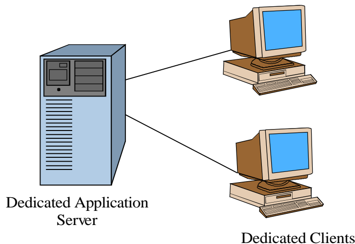
FIG. 1: TWO-TIER ARCHITECTURE
