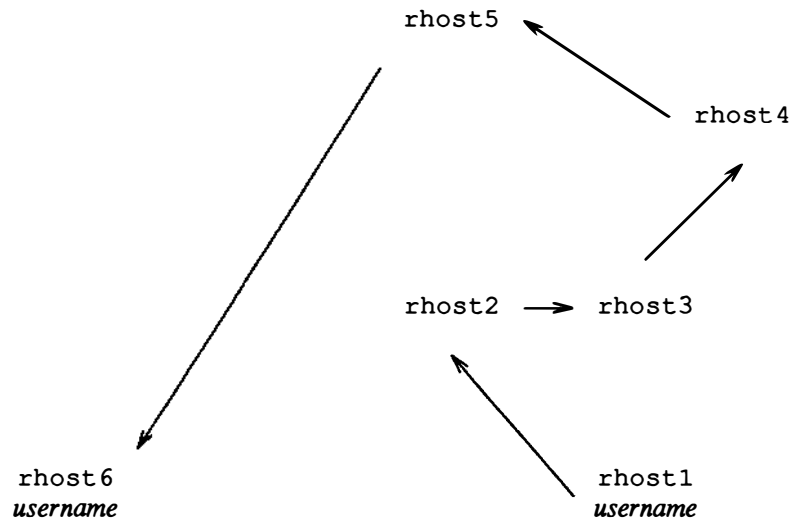
Figure 2-1. Sample indirect route with UUCP
