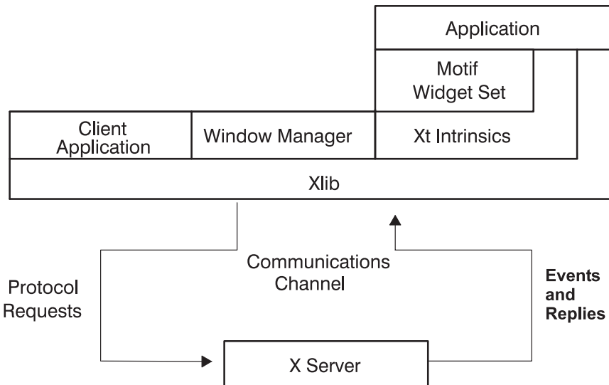
Figure 1. X-Windows Components
