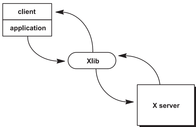
Figure 2. Xlib Data Flow
