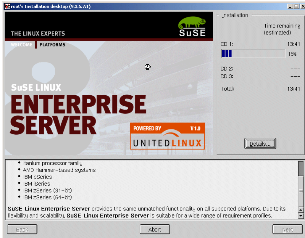
Figure 5-3 Software installation
