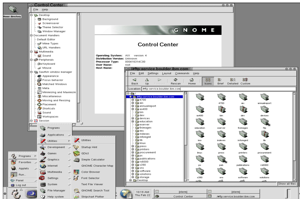
Figure 4-12 Gnome desktop
