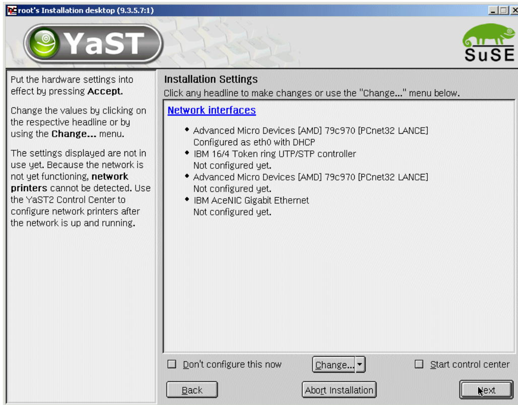
Figure 5-4 Network configuration
