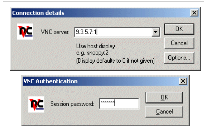
Figure 5-5 Start vncviewer
