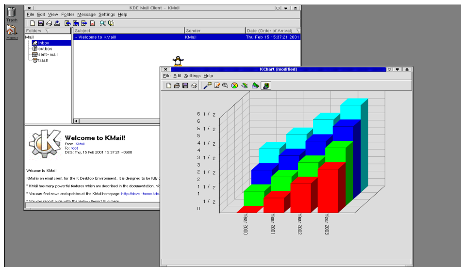
Figure 4-9 KOffice sample 2
