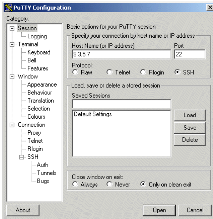
Figure 5-8 Connecting via ssh and PuTTY
