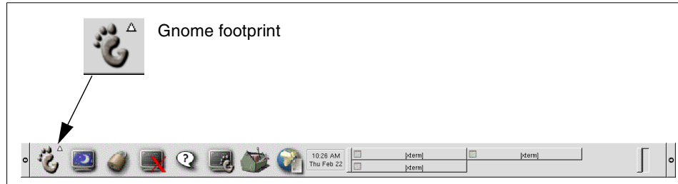
Figure 4-13 Gnome panel
