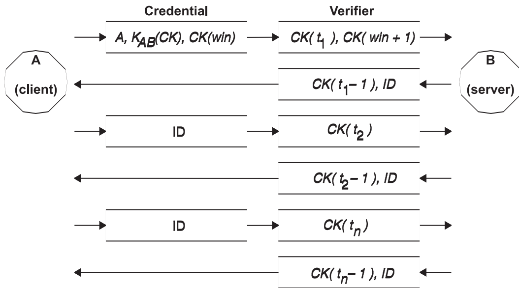
Figure 16. Authentication Process. This figure illustrates the authentication process.
