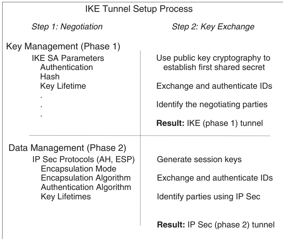
Figure 9. IKE Tunnel Setup Process. This illustration shows the two-step, two-phase process for setting up an IKE tunnel.
