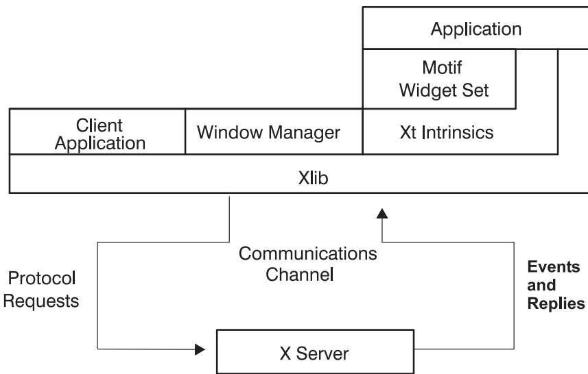
Figure 1. X-Windows Components
