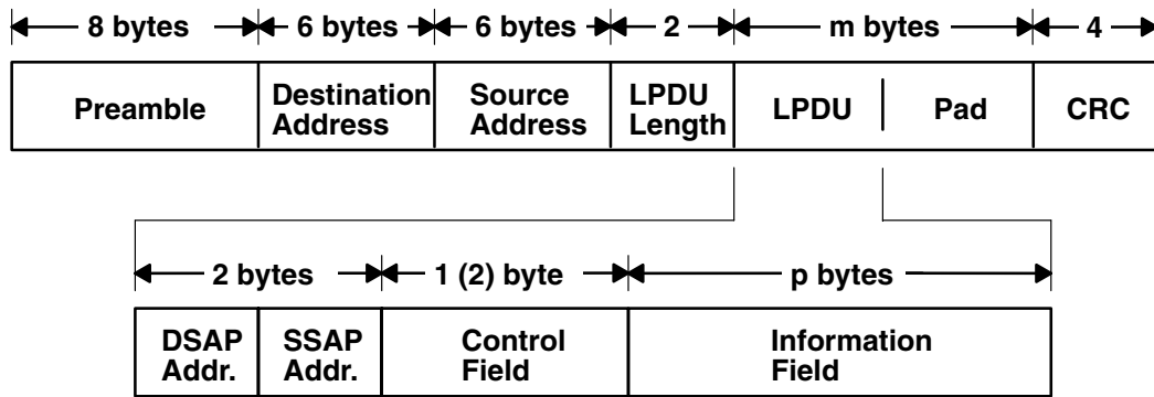
Figure 6. A Block. This diagram shows the DLC8023 data packet containing the following: preamble (8 bytes), destination address (6 bytes), source address (6 bytes), LPDU length (2 bytes), LPDU, Pad (together with LPDU consist of m bytes), and CRC (4 bytes). A second line shows that LPDU consists of the following: DSAP address, SSAP address (together with DSAP address consist of 2 bytes), control field [1 (2) byte], and the information field ( p bytes).
