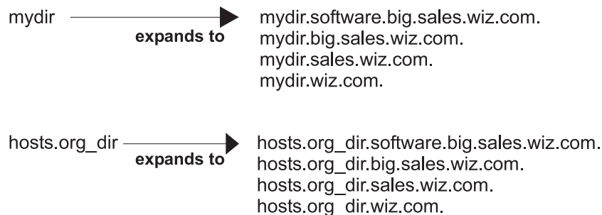
Figure 17. Partly Qualified Name Expanding to Fully Qualified Name. This illustration shows partly qualified names expanding to fully qualified names. hosts.org_dir , for example, expands to hosts.org_dir.software.big.sales.wiz.com. , hosts.org_dir.sales.wiz.com. , hosts.org_dir.wiz.com.
