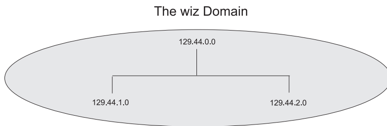
Figure 4. Example NIS Domain. An example domain, named wiz, with one server IP address and two subordinate workstation IP addresses.
