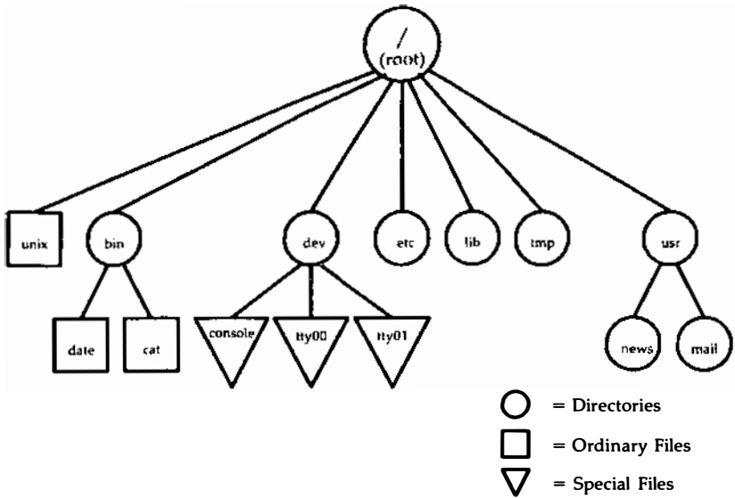
Figure 3-1: A Sample File System
