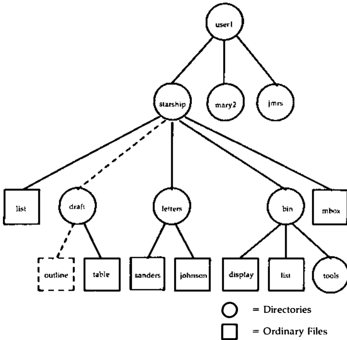
Figure 3-6: Relative Path Name from starship to outline
