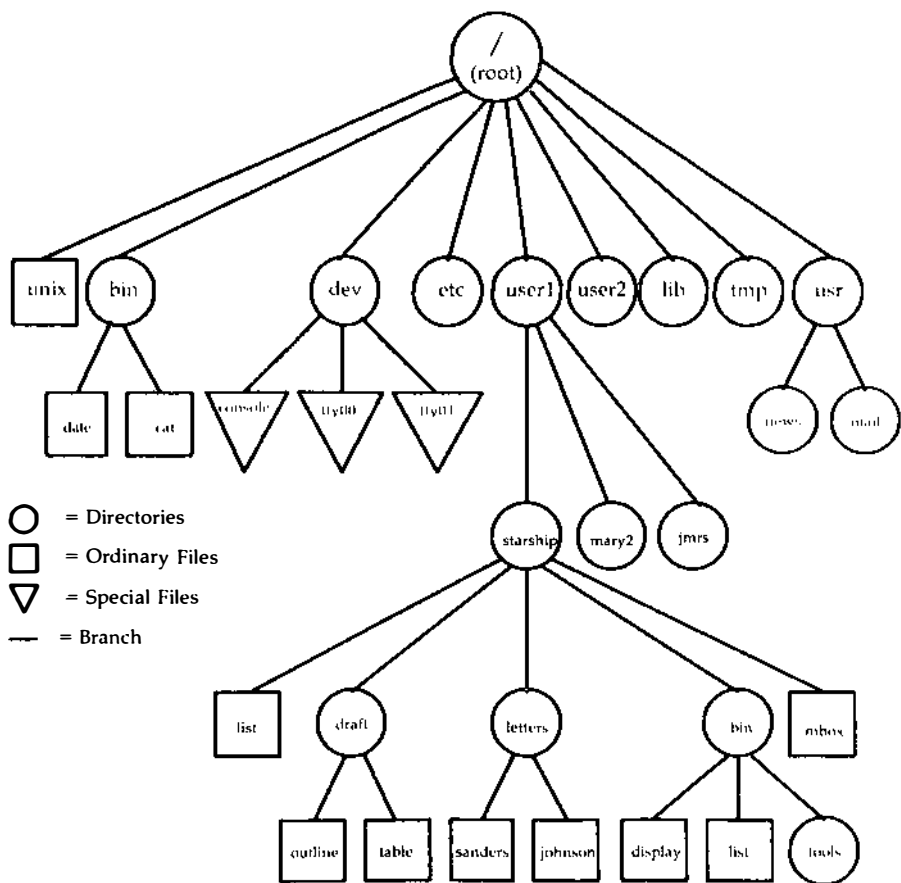
Figure 3-2: Directory of Home Directories
