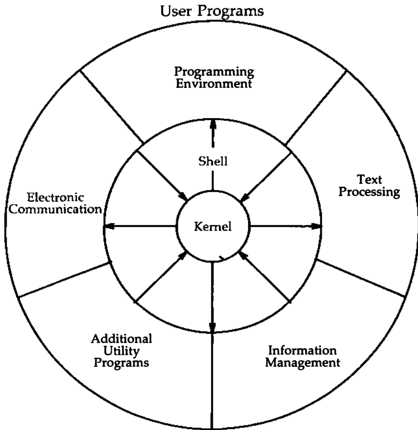
Figure 1-1: Model of the UNIX System
