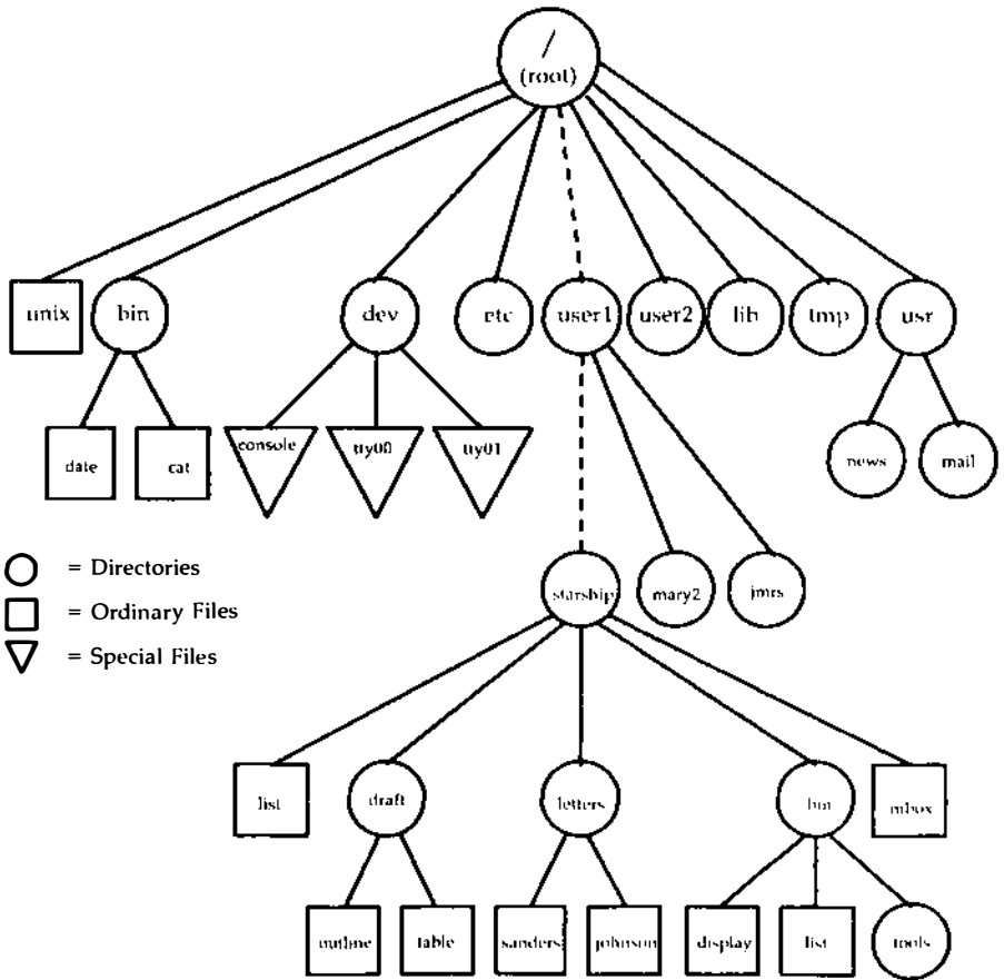
Figure 3-4: Full Path Name of the /user1/starship Directory
