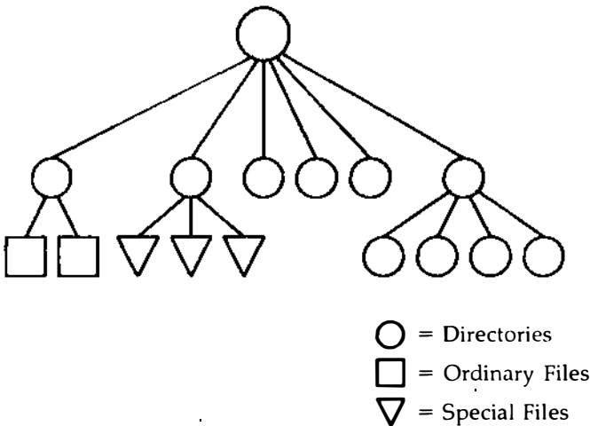
Figure 1-3: The Hierarchical Structure of the File System
