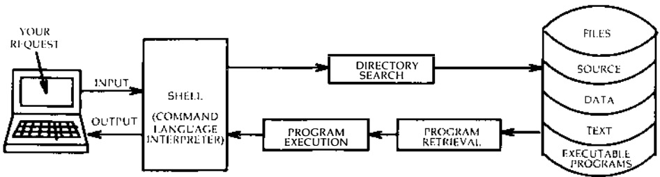
Figure 1-5: Execution of a UNIX System Command
