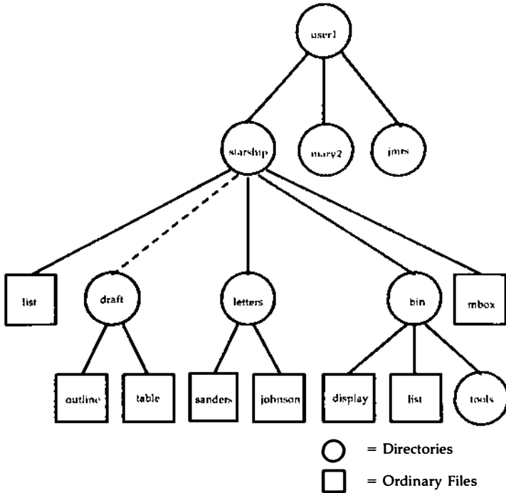
Figure 3-5: Relative Path Name of the draft Directory
