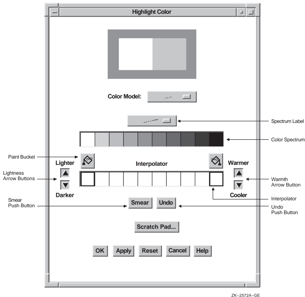
Figure 6–1 Components of the ColorMix Widget (Color Picker Model)
