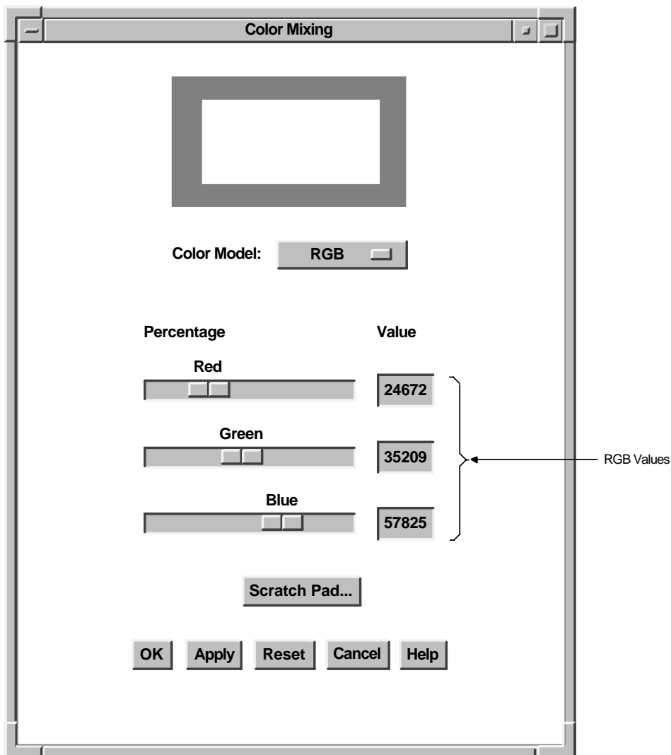
Figure 6-3 Components of the ColorMix Widget (RGB Color Model)
