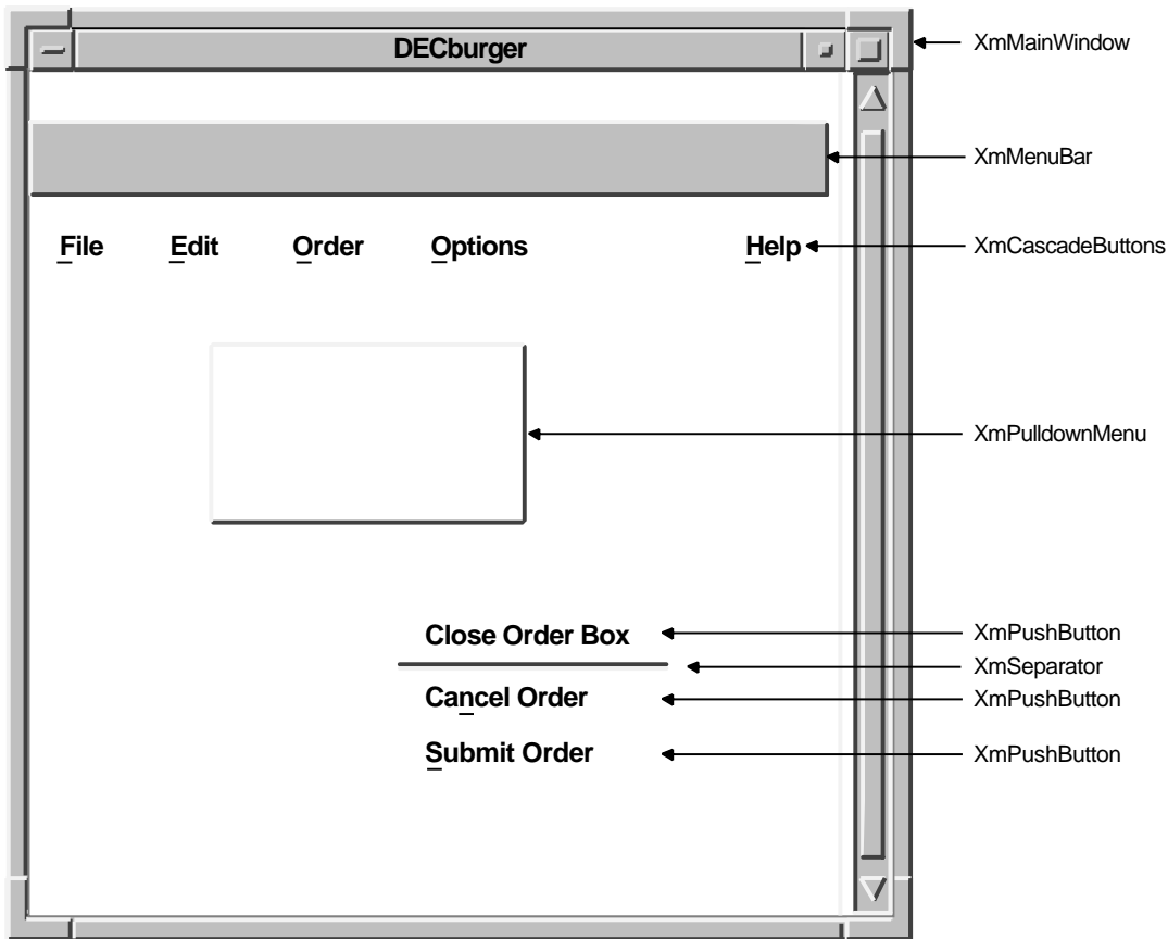
Figure 1–2 The OpenVMS DECburger Widget Hierarchy
