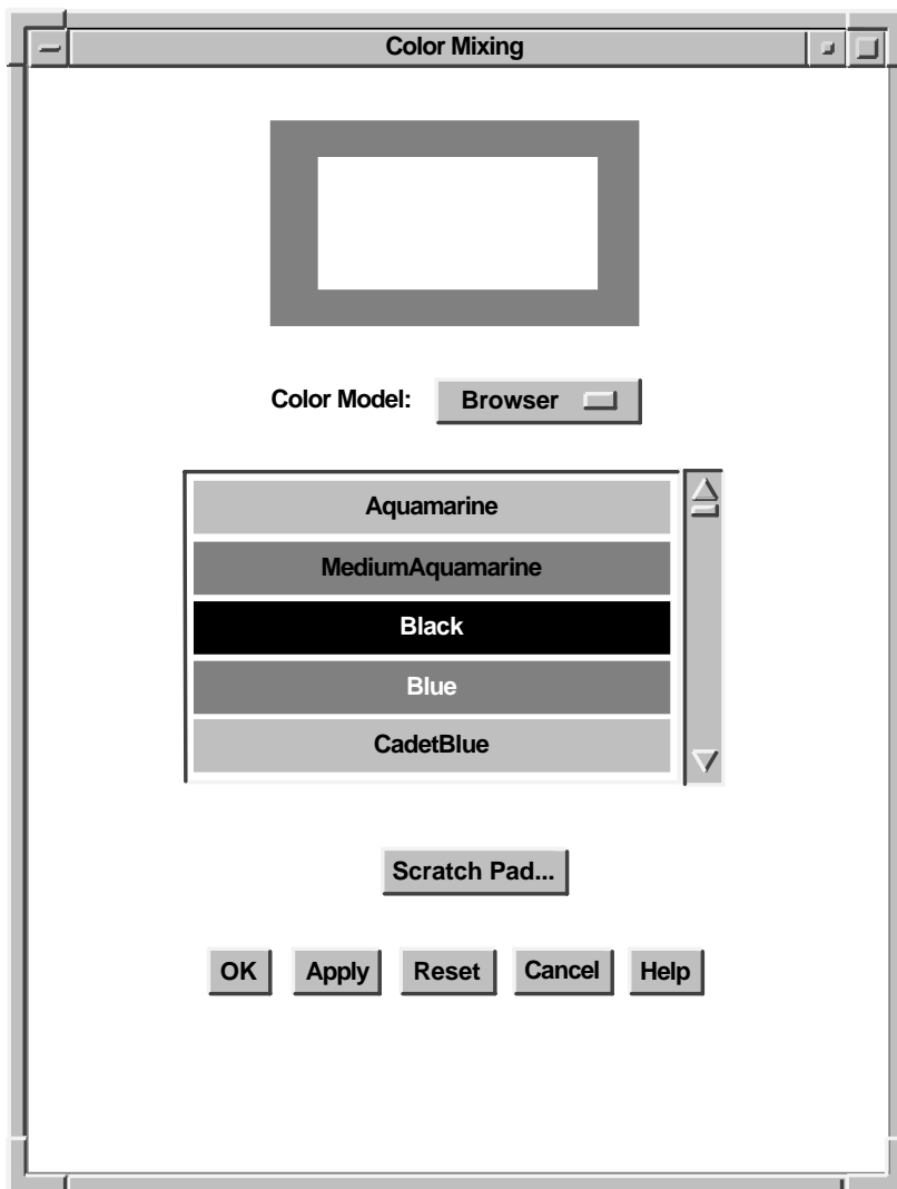
Figure 6–4 Components of the ColorMix Widget (Browser Color Model)
