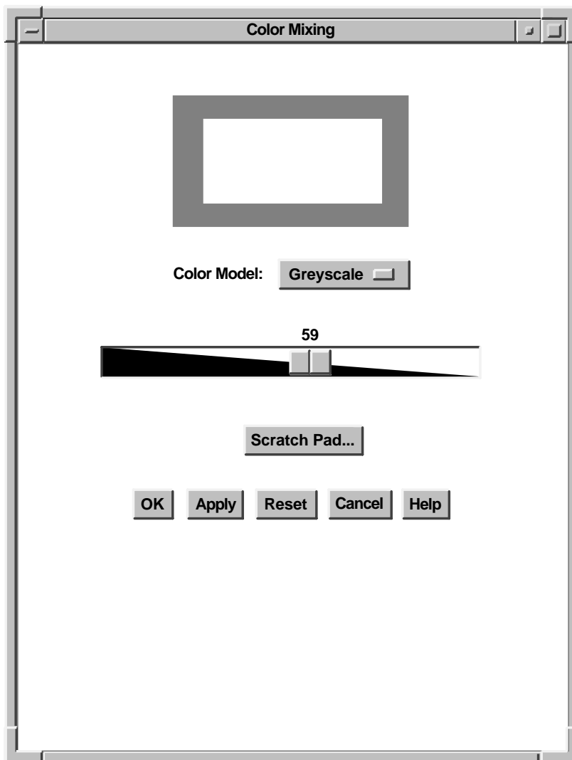
Figure 6-5 Components of the ColorMix Widget (Greyscale Mixer)
