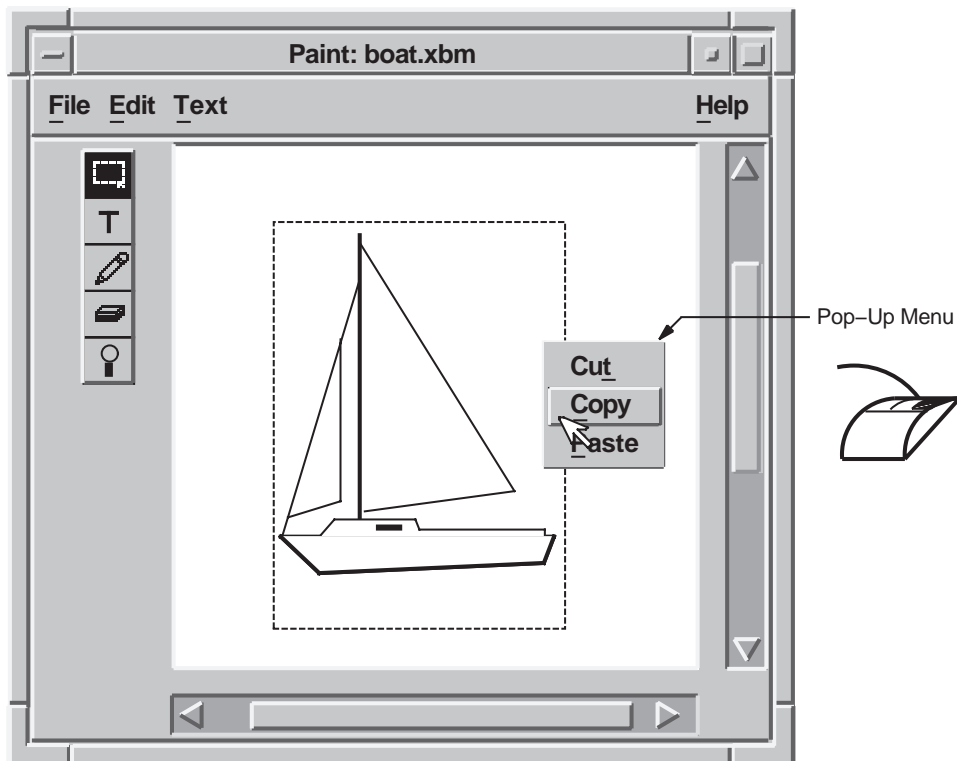
Figure 2-6 Pop-up Menu
