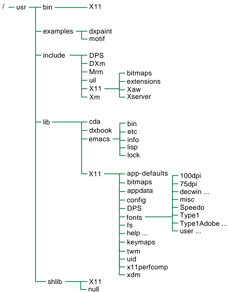
Figure B-2: X Directory Structure
