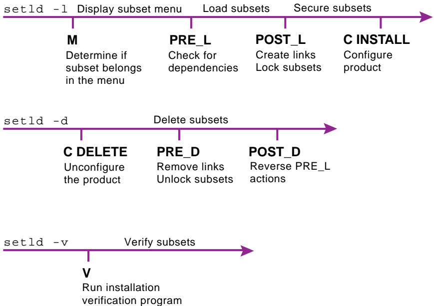
Figure 3–1: Time Line of the setld Utility
