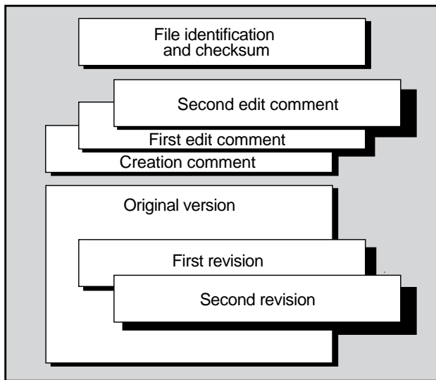
Figure 6-1: Contents of a Version Control File
