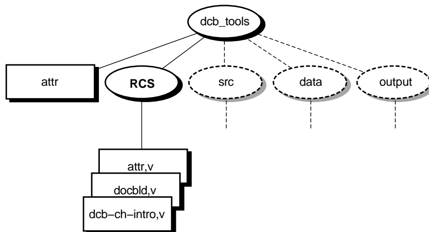
Figure 6-2: A Typical RCS Library
