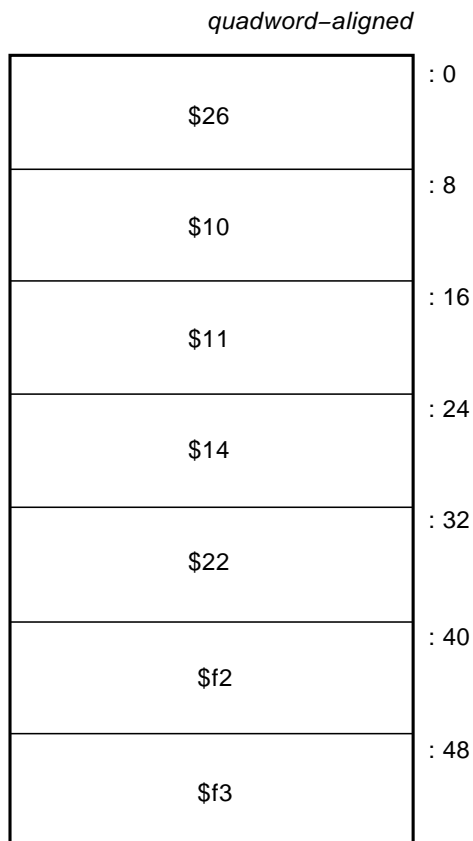
Figure 3–4: Register Save Area Example
