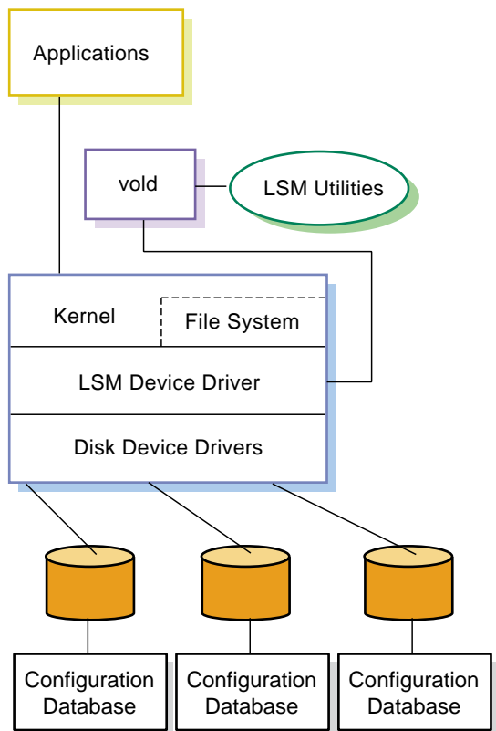
Figure 1–9: LSM Architecture
