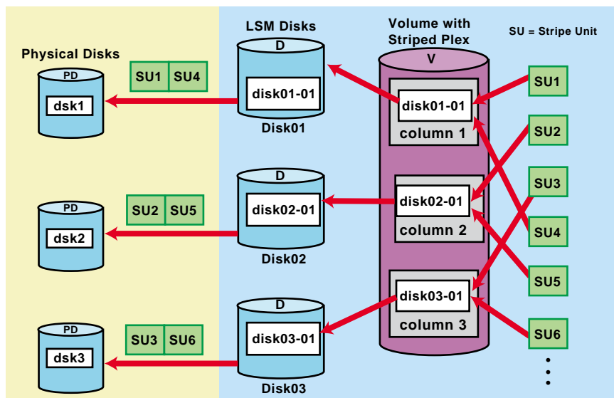
Figure 1–4: Example of a Striped Volume
