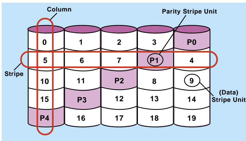
Figure 1-6: Left-Symmetric Layout
