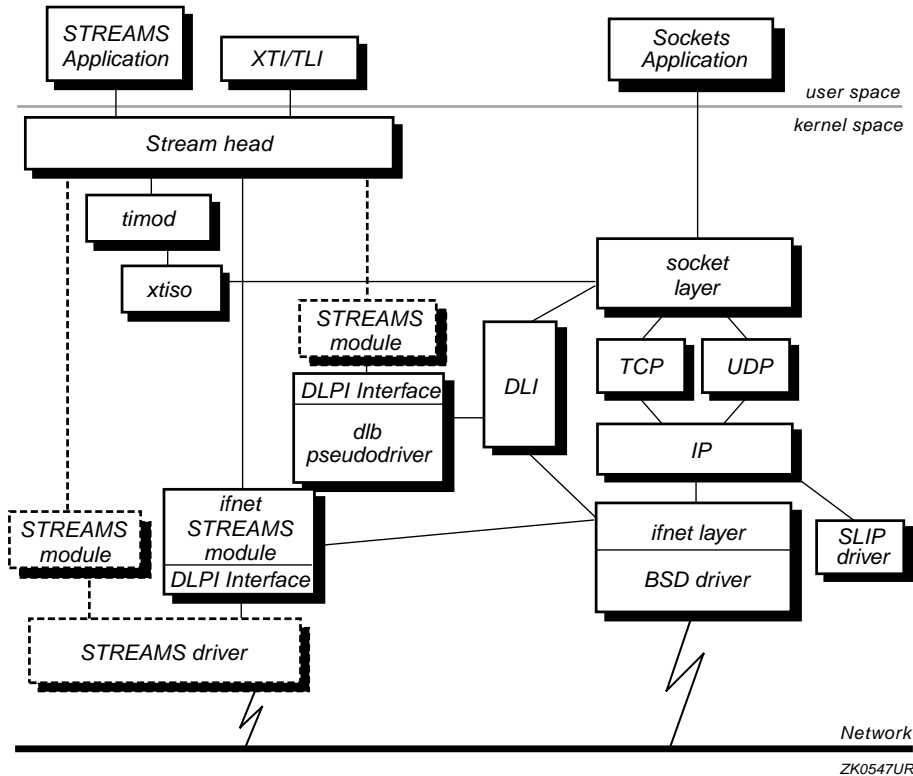
Figure 3–2: Frameworks XTI, STREAMS and Sockets Interactions
