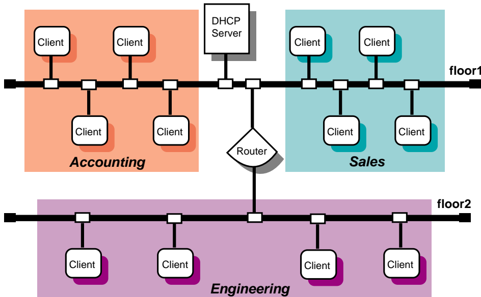
Figure 3–3: DHCP Configuration
