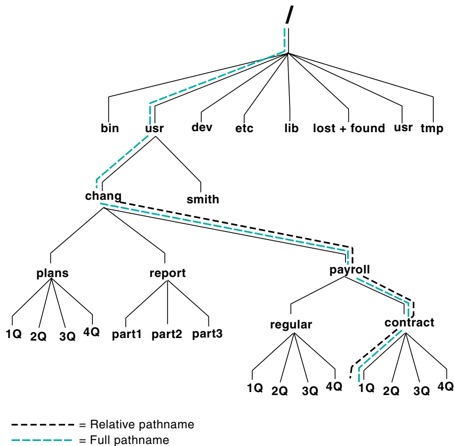
Figure 2–2: Relative and Full Pathnames
