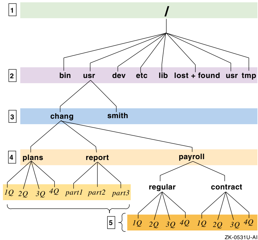
Figure 2–1: A Typical File System
