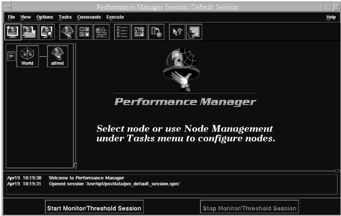
Figure 2 Main Window
