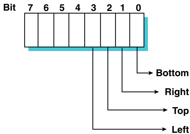
Figure D-2: Bit Pattern for DECDRLBR Parameters
