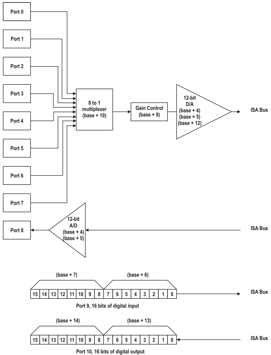
The PCL-711 card, with register offsets.
