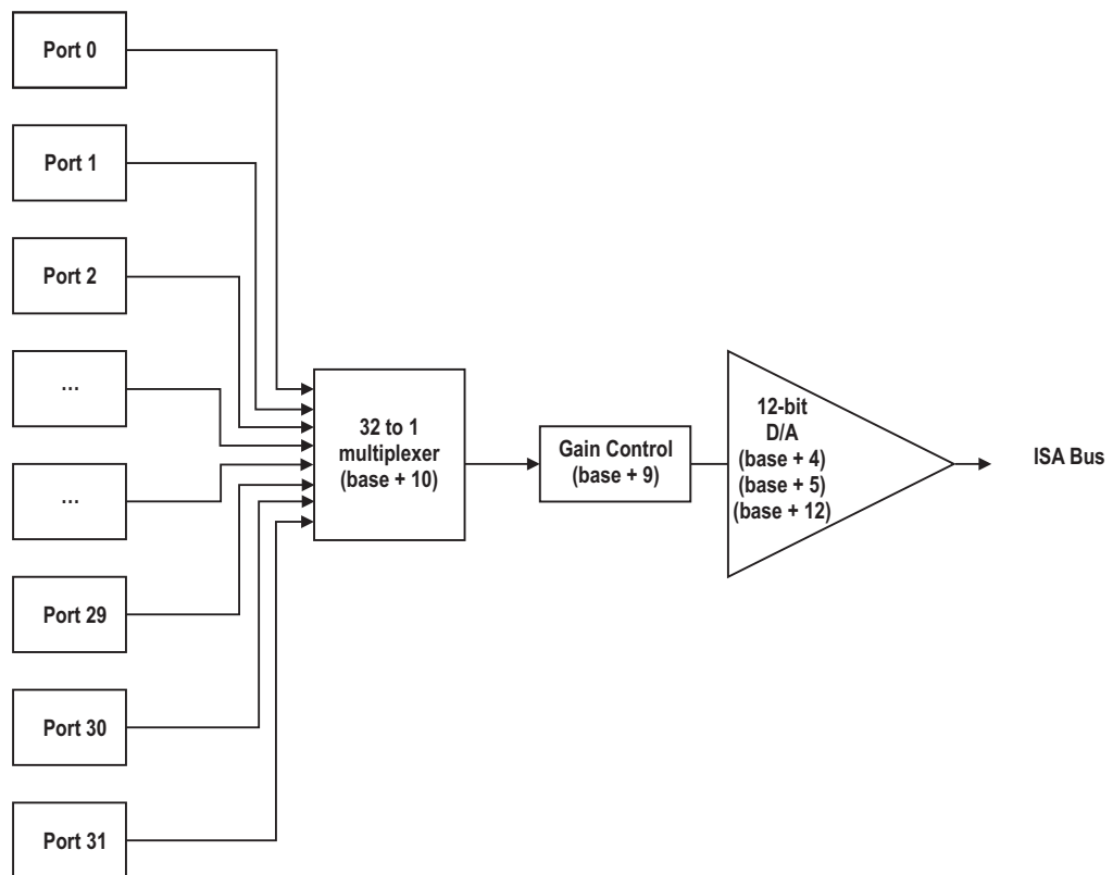
The ISO-813 card high-level view with register offsets.
