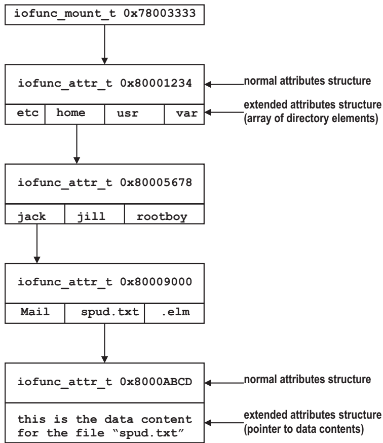
Internal resource manager view of a filesystem.
