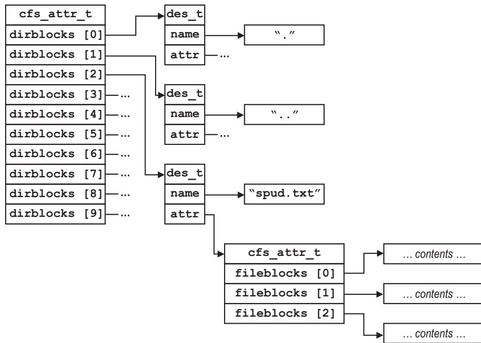
A directory, with subdirectories and a file, represented by the internal data types.
