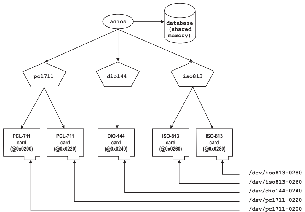
The relationship between ADIOS, the shared memory database, the hardware drivers, and their cards.
