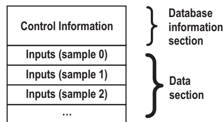
The shared memory layout.
