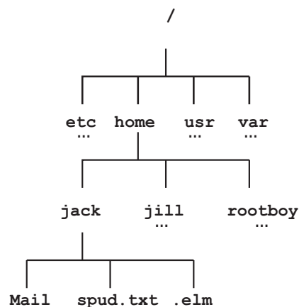
A small portion of a filesystem tree.
