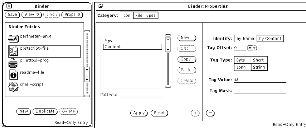
Figure 16-11 The postscript-file Content File Type Entry
