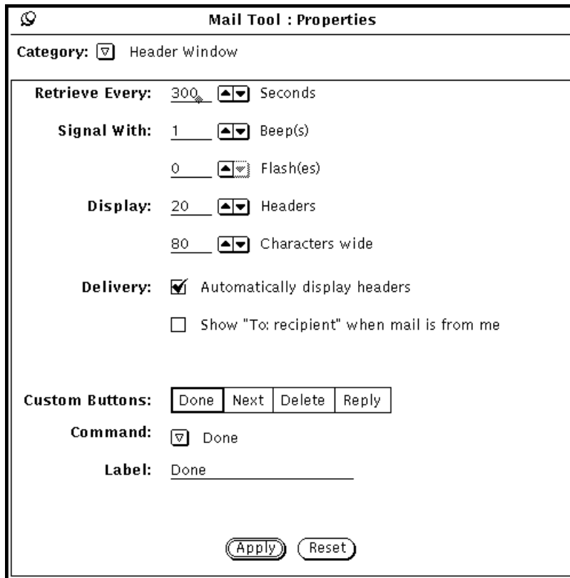
Figure 4-31 Header Window Properties
