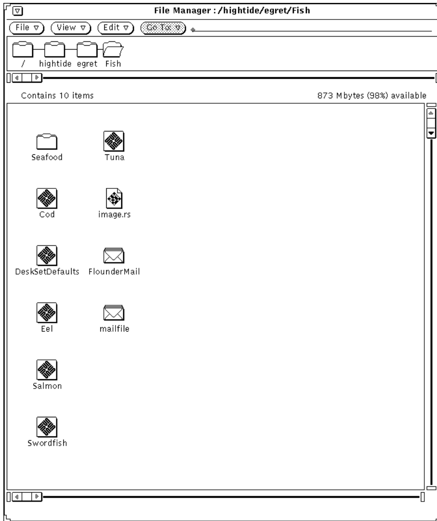
Figure 2-39 Icons Listed in Columns (Vertically) in the File Pane
