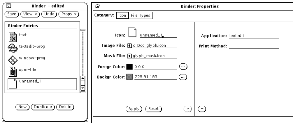
Figure 16-13 A New Binder Entry
