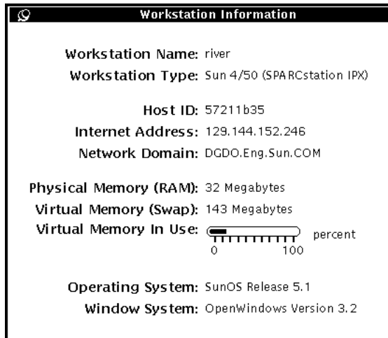
Figure 17-1 Workstation Information Window
