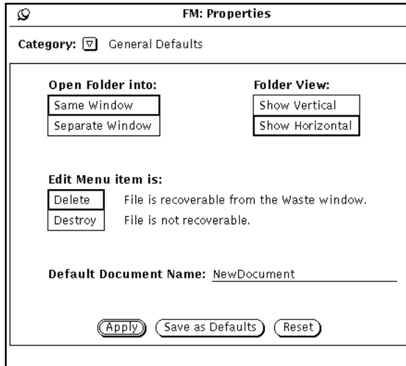
Figure 2-34 General Defaults Properties Window
