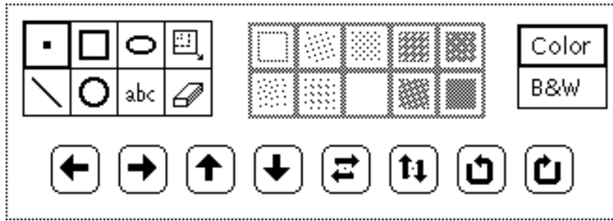
Figure 15-3 Icon Editor Drawing Controls
