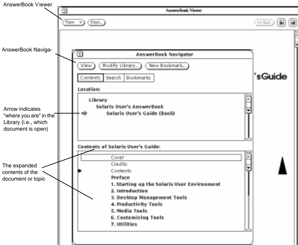
Figure 19-1 Documentation in the Navigator and Viewer
