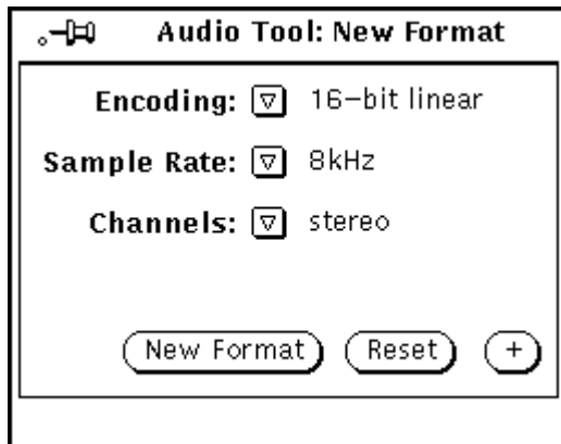
Figure 11-13 Audio Tool: New Format Window
