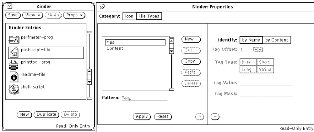
Figure 16-10 The *.ps File Type Entry
