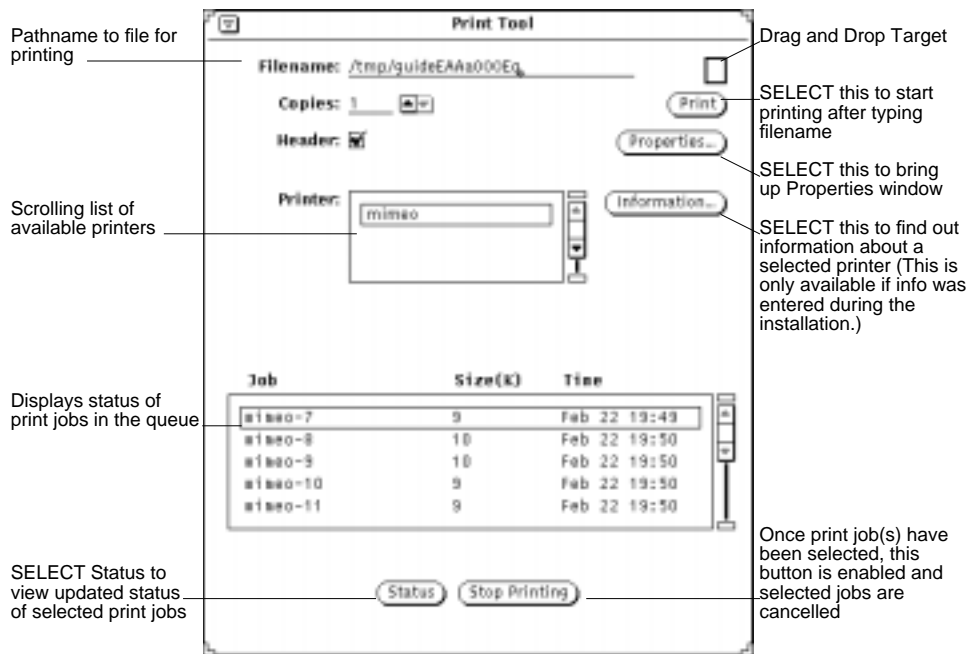
Figure 10-2 Print Tool Window
