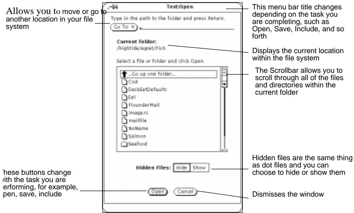
Figure 1-26 An example of the Open Window
