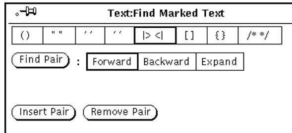
Figure 3-7 Text: Find Marked Text Pop-up Window
