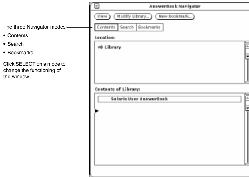
Figure 19-2 AnswerBook Navigator in Contents Mode
