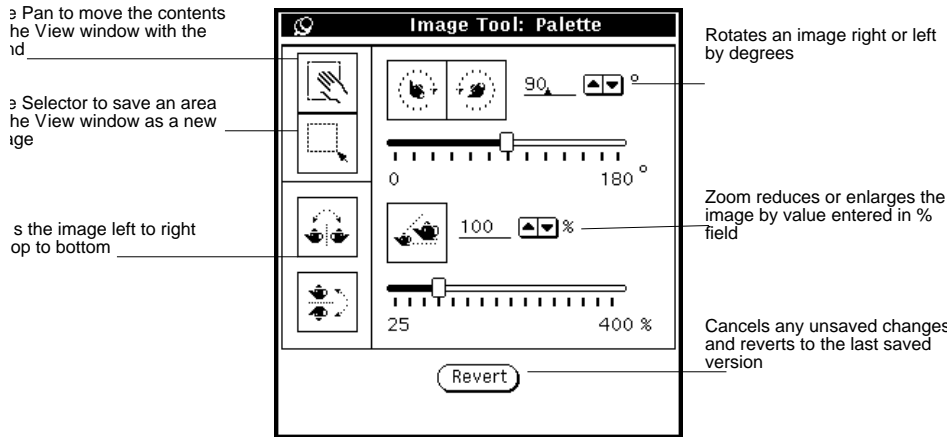
Figure 13-7 Image Tool Palette
