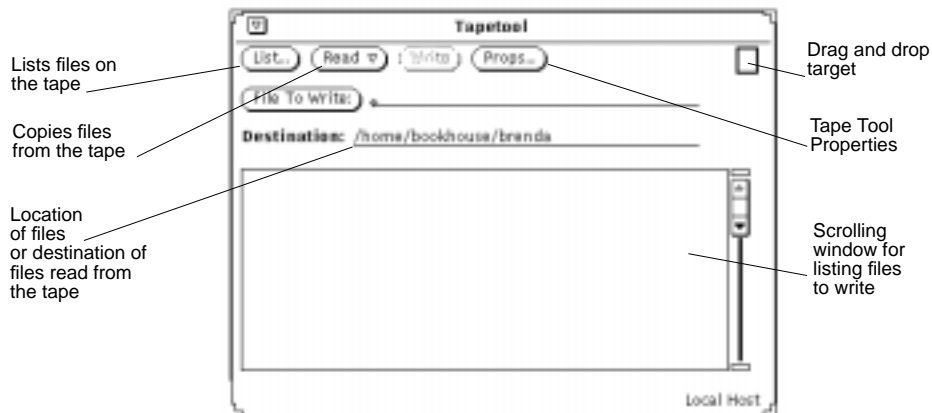
Figure 12-2 Tape Tool Window
