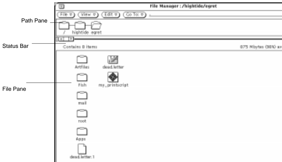
Figure 2-2 Primary File Manager Window
