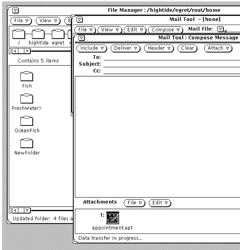
Figure 2-20 Dragging a Mail Attachment onto File Manager
