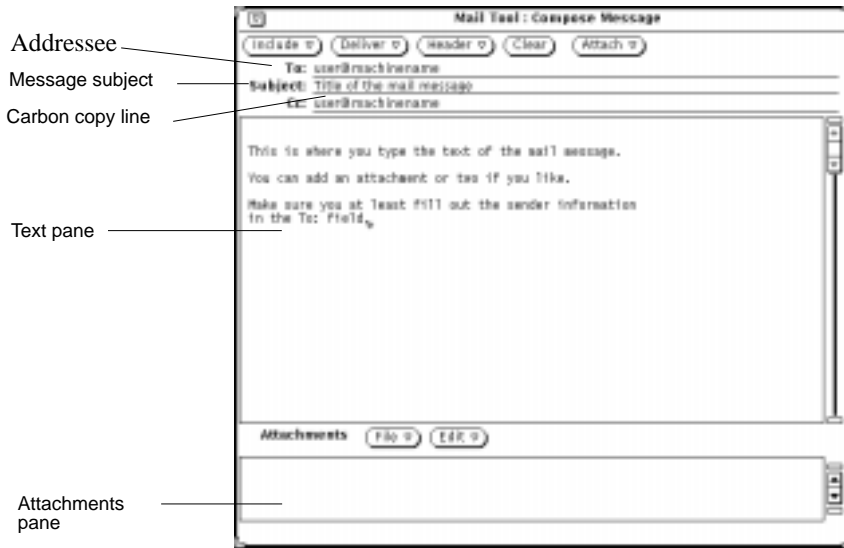
Figure 4-12 Addressing a Message
