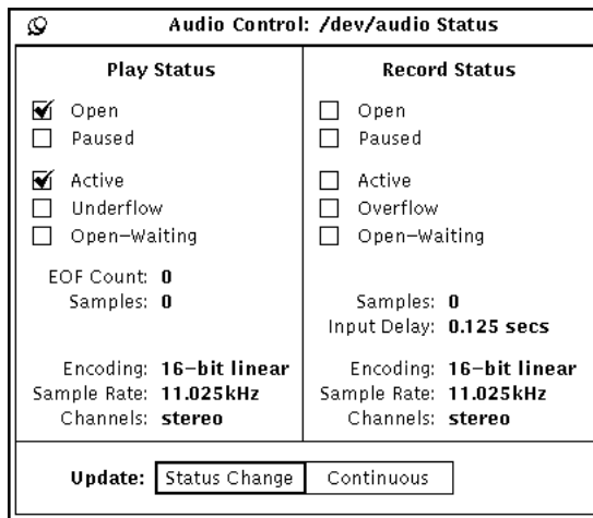
Figure 11-23 Audio Control: Status Window
