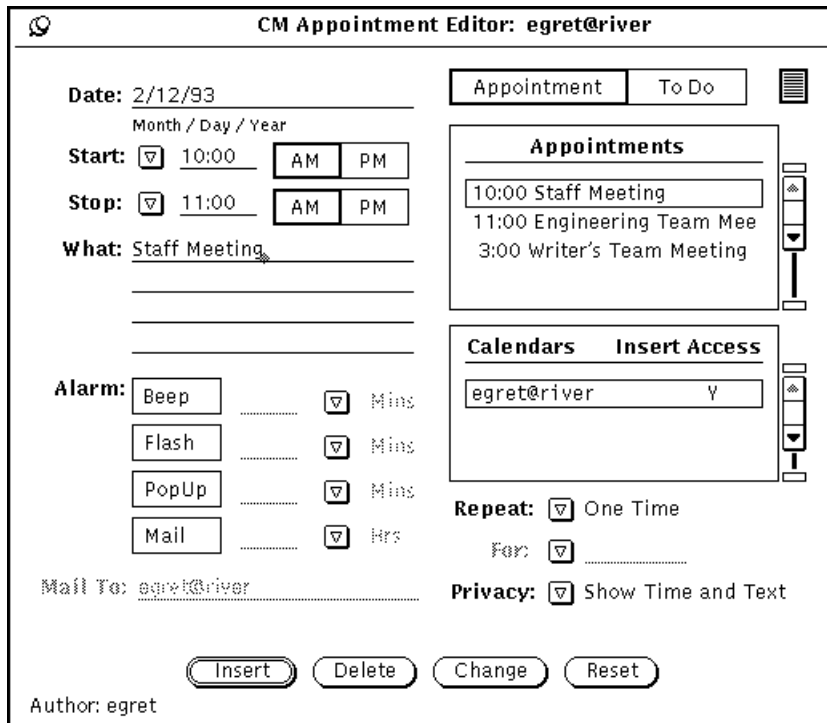
Figure 5–11 Appointment Editor Window with a Highlighted Appointment
