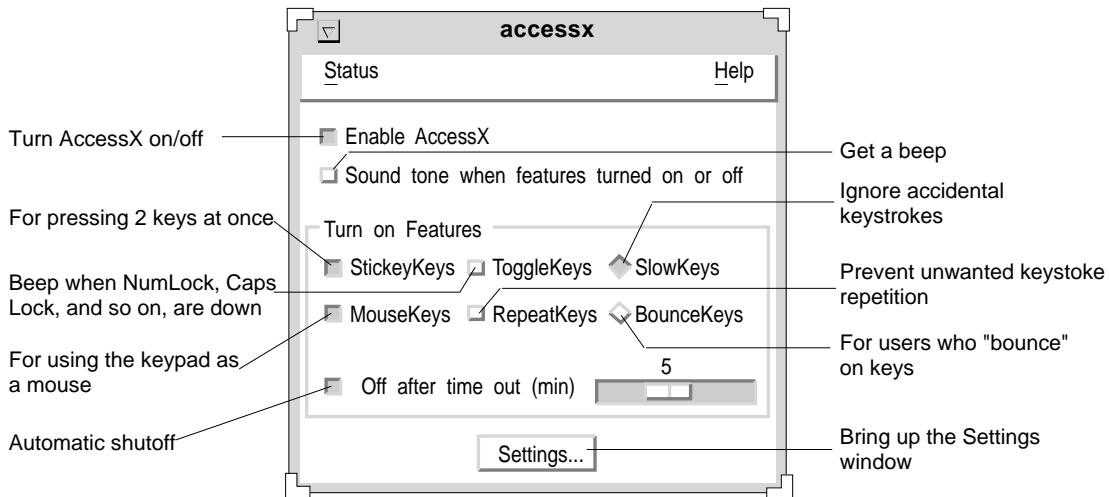
Figure B-1 The AccessX Main Window
