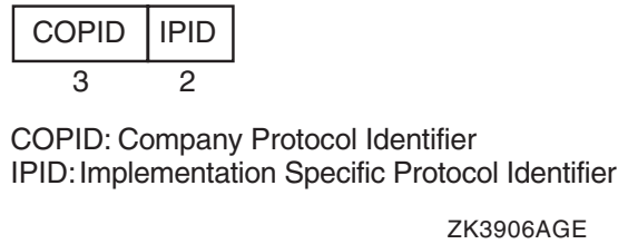
Figure 9-11 802.1 Header Subfields
