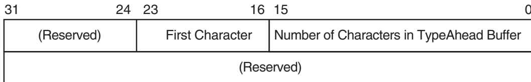
Figure 5-12 Sense Mode Characteristics Buffer (type-ahead)
