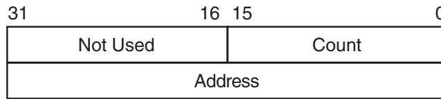
Figure 1-2 ACP Device/Function Argument Descriptor Format
