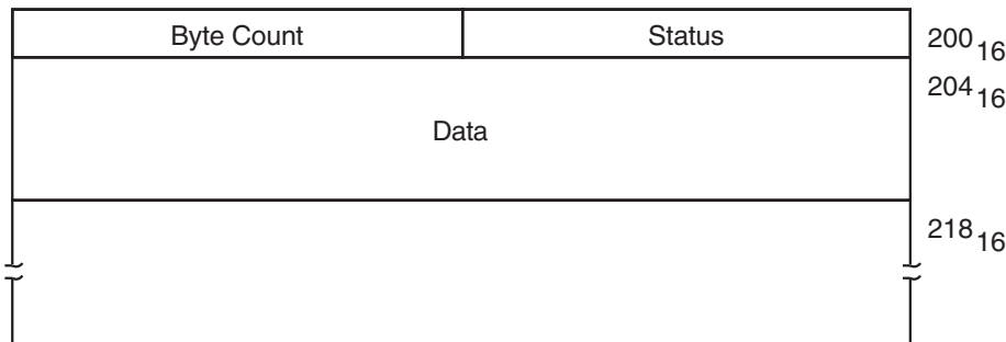
Figure 6-1 Buffer Layout
