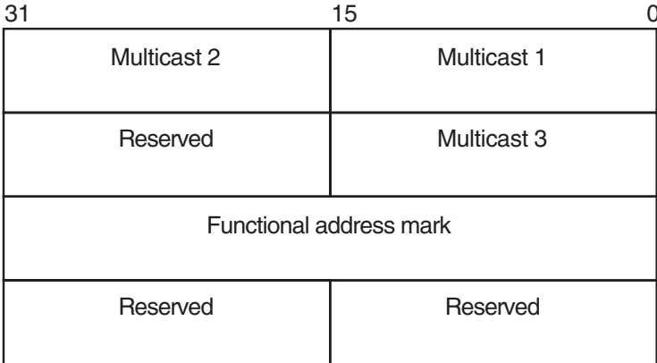
Figure 9-28 Format of IO$M_SHOW_MAP P2 Buffer
