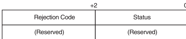
Figure 5-18 IOSB Contents—LAT Port Driver Function
