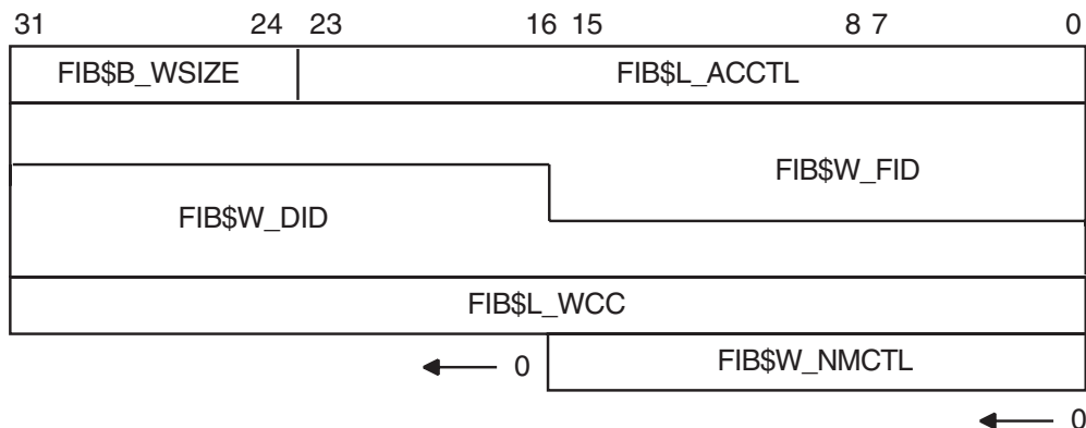
Figure 1-3 Typical Short FIB
