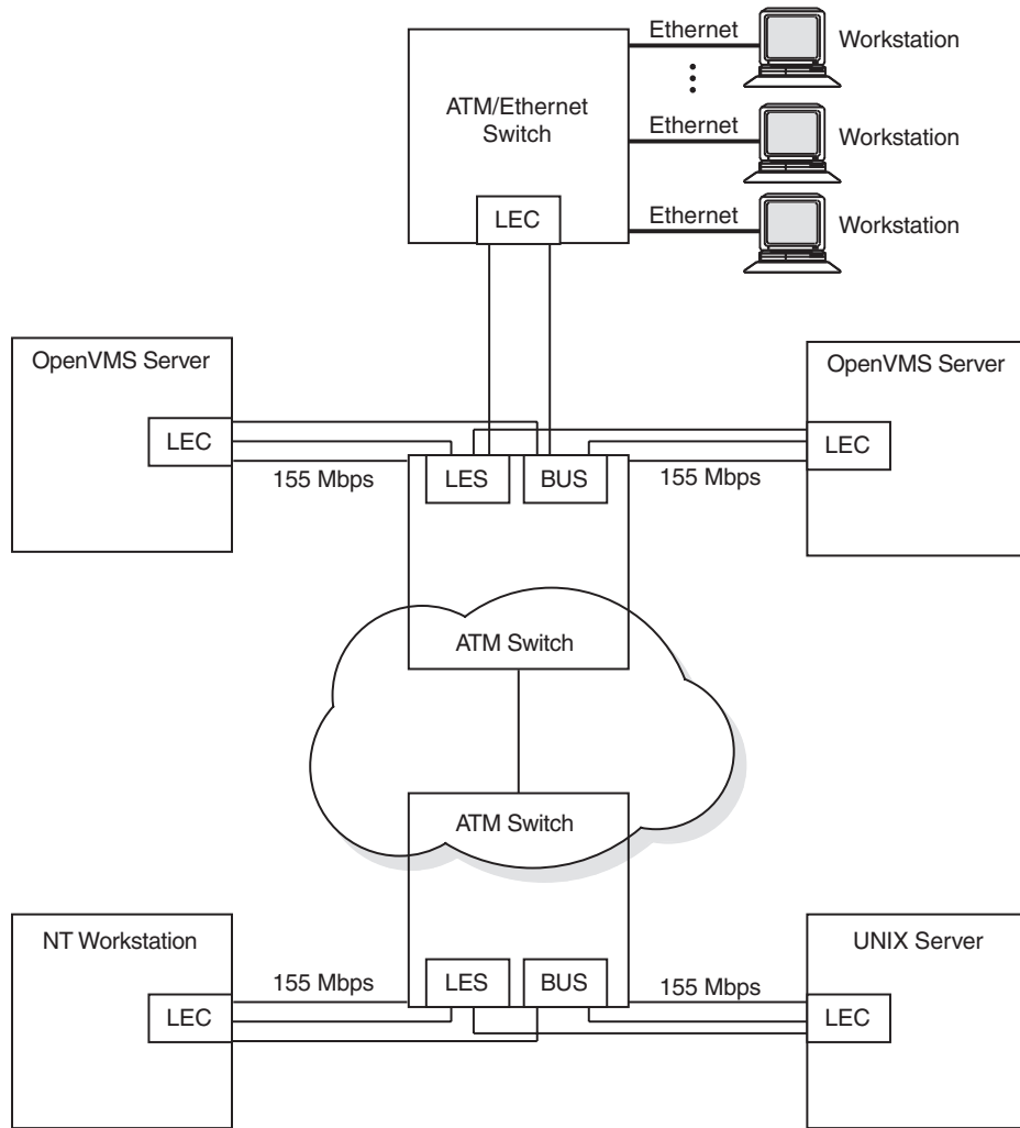
Figure 9-1 Emulated LAN Topology
