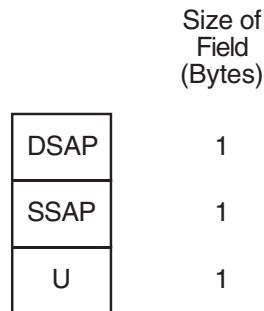
Figure 9-16 Class I Service 802.2 Header
