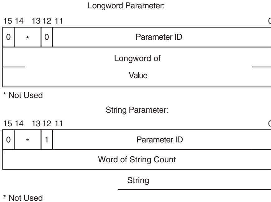
Figure 9-27 Sense Mode Attribute Buffer
