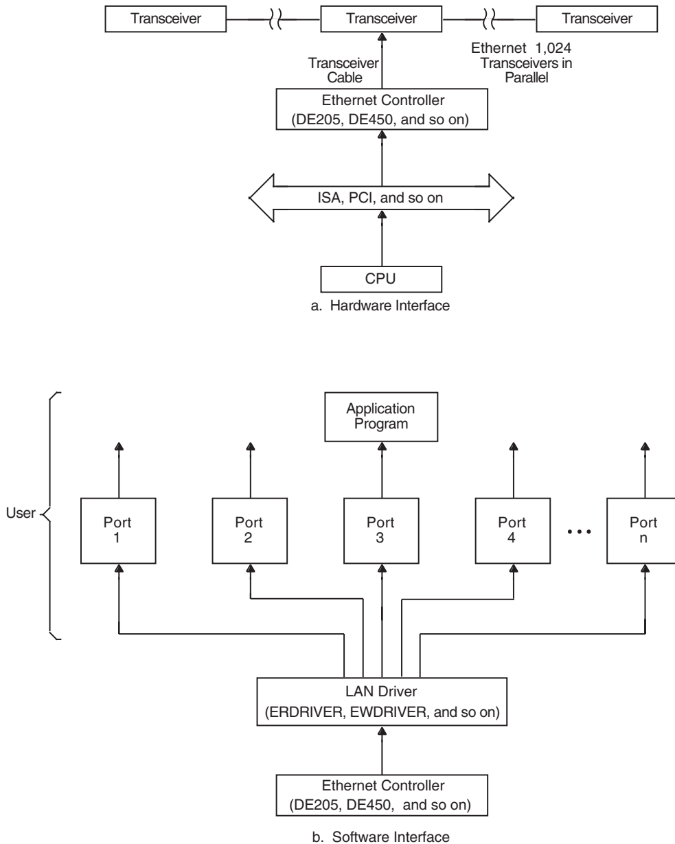
Figure 9-2 Typical Ethernet Configuration
