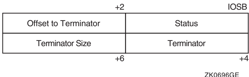
Figure 5-14 IOSB Contents—Read Function
