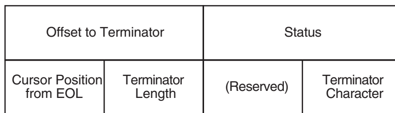
IOSB Contents: Itemlist Read Function
