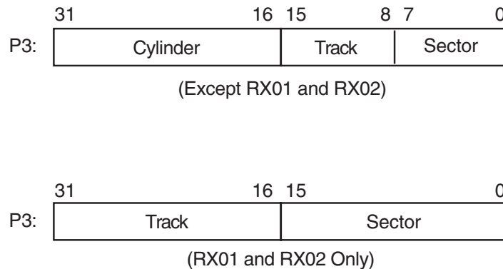
Figure 2-1 Disk Physical Address
