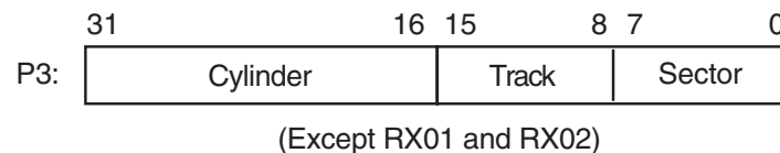
Figure 2-5 Starting Physical Address
