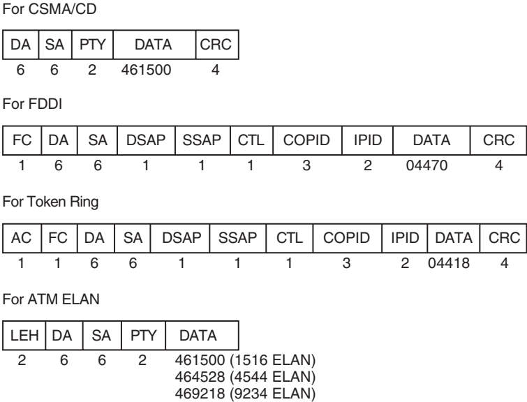
Figure 9-13 Frames with Ethernet Format
