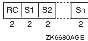
Figure 9-12 Source Routing Field (Alpha Only)
