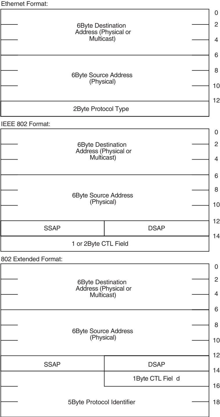
Figure 9-21 Read Function P5 Buffer
