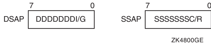
Figure 9-18 DSAP and SSAP Format
