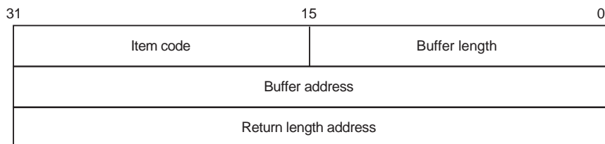
Figure 11–1 Item Descriptor Data Structure
