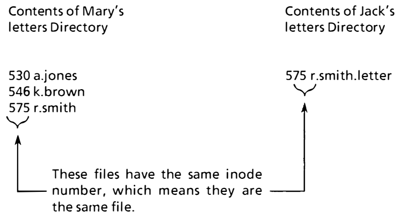
Figure 2-17. Links to a File
