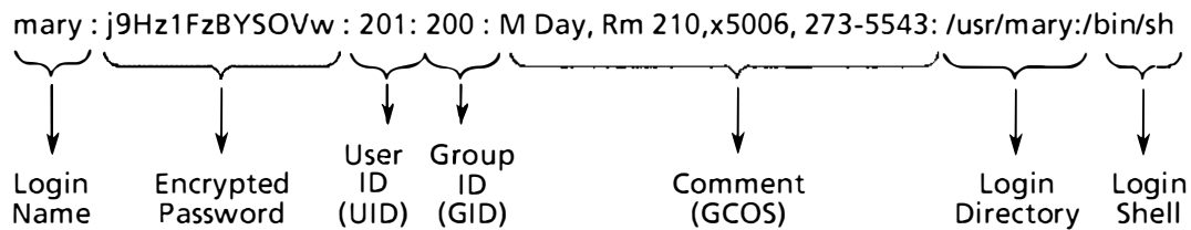
Figure 3-2. Sample Entry in the /etc/passwd File
